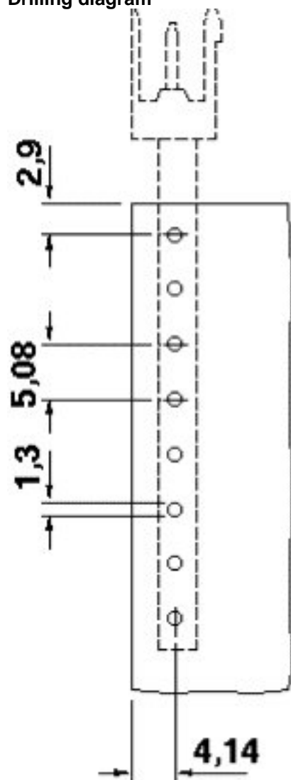
Drilling diagram
